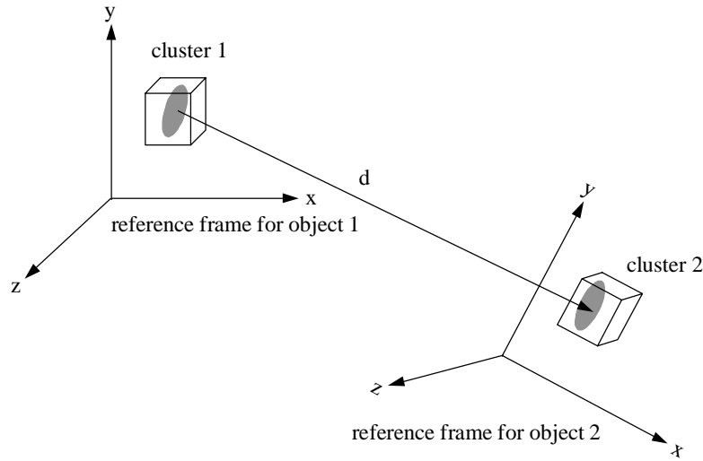
Figure 4. Configuration to estimate the form factor between two clusters.
